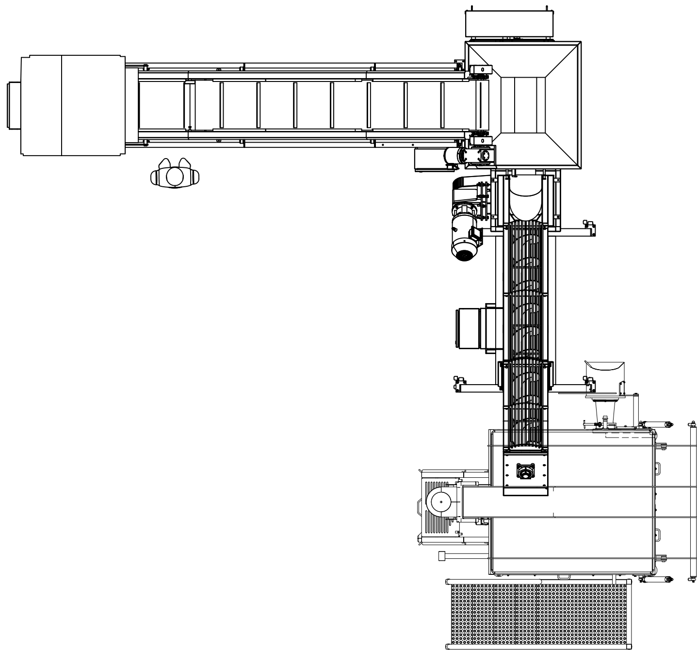
VIEW SHOWING SCREW AUGER IN LOADING POSITION
