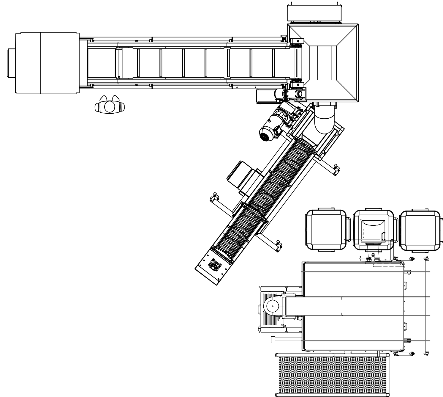
VIEW SHOWING SCREW AUGER MOVED TO LOAD BUGGIES
